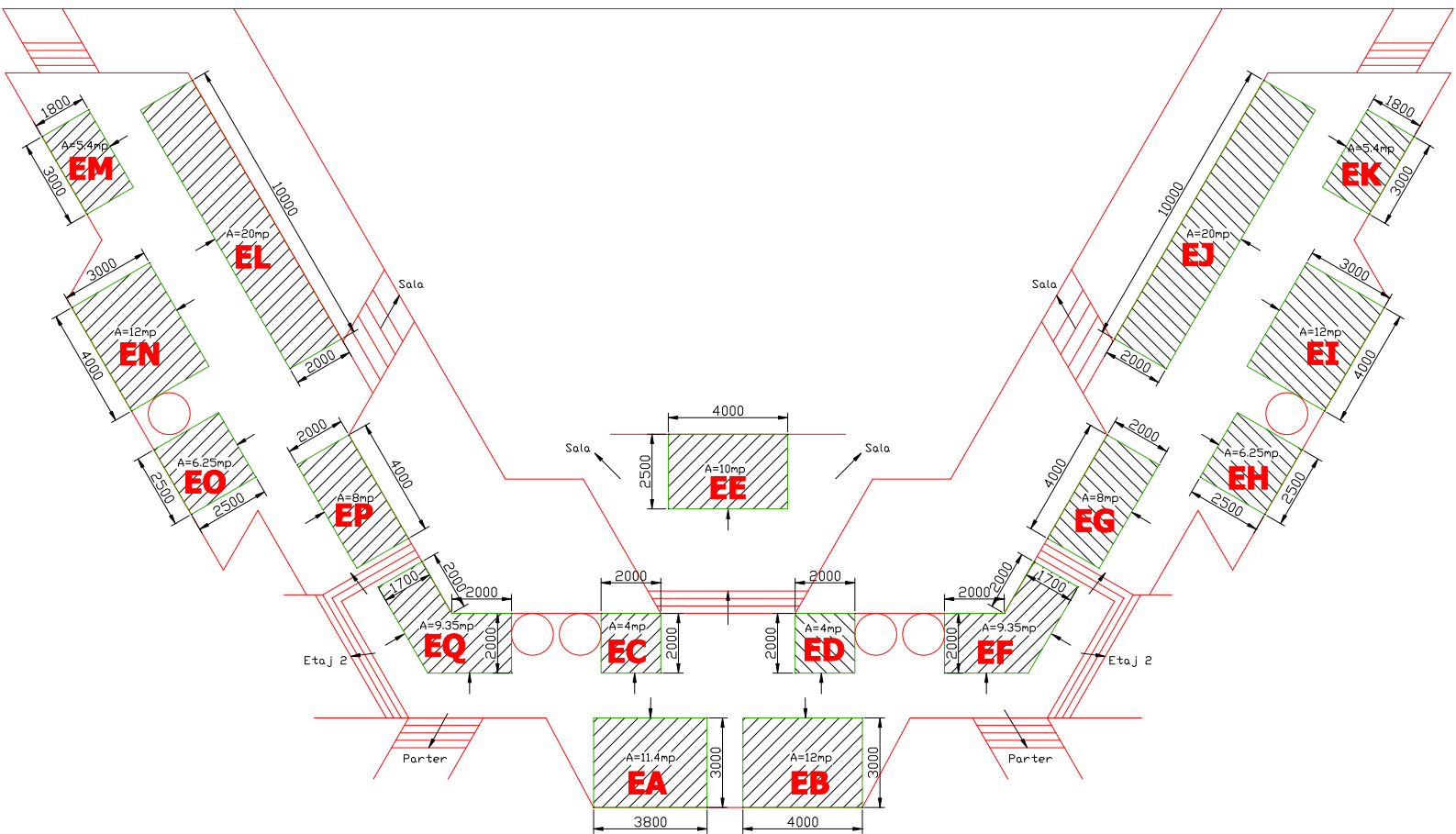
Plan Etaj 1 Suprafata totala standuri A=163.4\text{mp}
